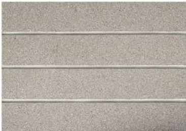
Code:S21 dimensions :100x600x27
